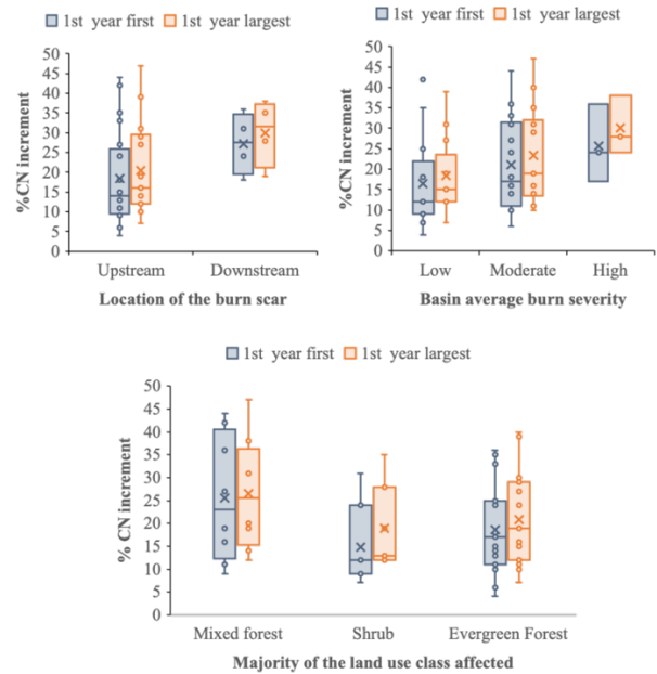
Fig. 3. Post-fire % CN increment under different fire characteristics, for 1st and largest peak flow events in immediate post-fire year.
