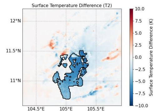
Fig. 4. Surface temperature difference between the baseline simulation and the second wetland approach
