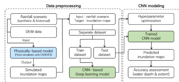
Fig. 1. Flowchart of the deep learning-based urban flood modeling
